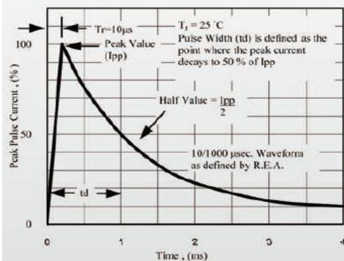
Fig. 5 - Pulse Waveform
